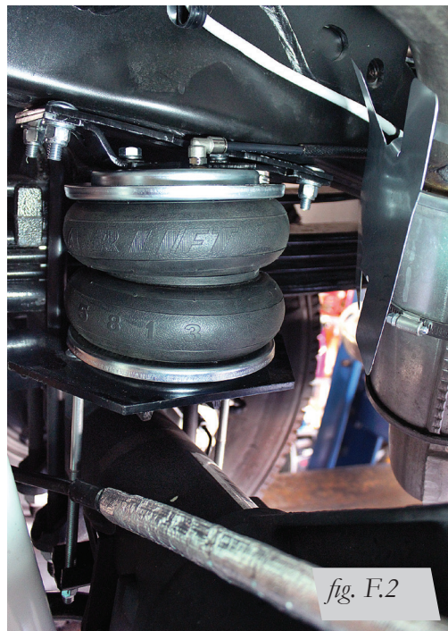
fig. F.2 Passenger's (right) side inside frame view of kit installed.
