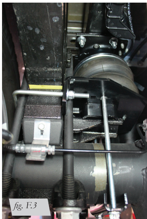
fig. F.3 Driver's (left) rear view of kit installed.
