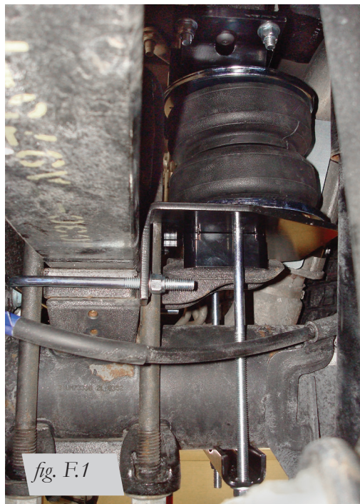
fig. F.1 Passenger's (right) side front view of kit installed.
