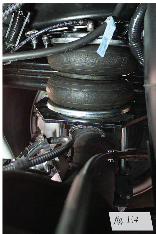
fig. F.4 Driver's (left) side inside frame view of kit installed.
